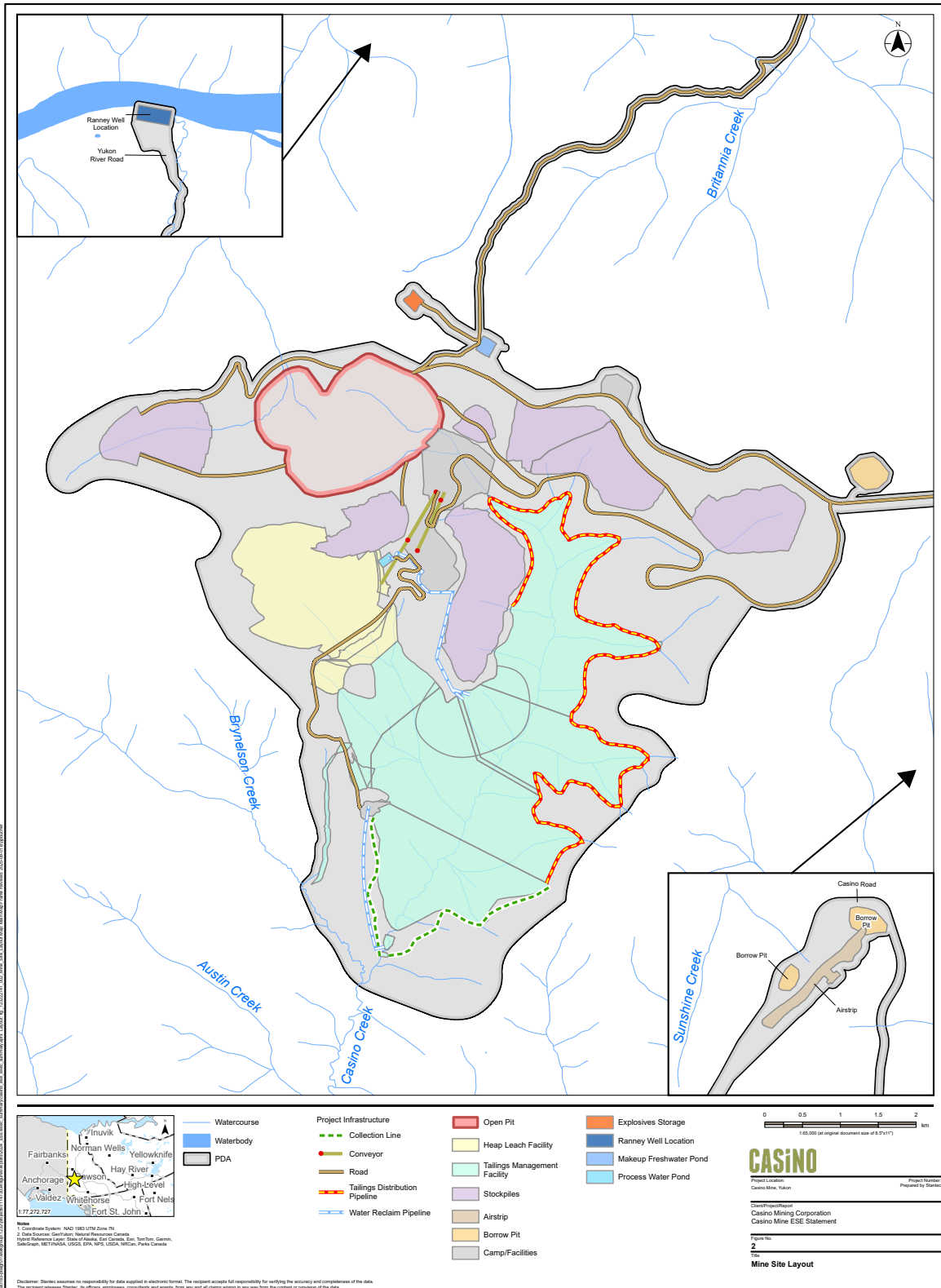
Figure ES.2 Casino Project Mine Site General Arrangement
